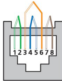
Conductor layout according to TIA/EIA 568A
