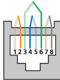
Conductor layout according to TIA/EIA 568B
