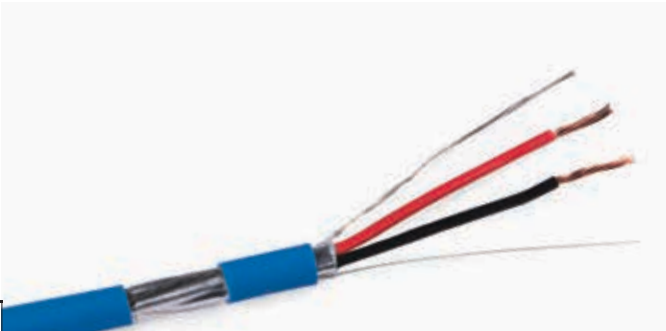
Shielded Multi-Conductor, 16/2, 65 Strand
