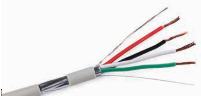
Shielded 18 AWG Multi-Conductor, 4 Conductor, Stranded Available in 500 FT Pull Box/1000 FT Reel, Riser & Plenum Part no. 18AWG-4C-STR-SH-QQQ-XX-YYYY
