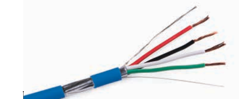
Shielded 22 AWG Multi-Conductor, 4 Conductor, Stranded Available in 500 FT Pull Box/1000 FT Reel, Riser & Plenum Part no. 22AWG-4C-STR-SH-QQQ-XX-YYYY
