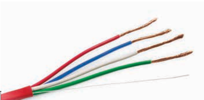
Unshielded 22 AWG Multi-Conductor, 4 Conductor, Stranded
