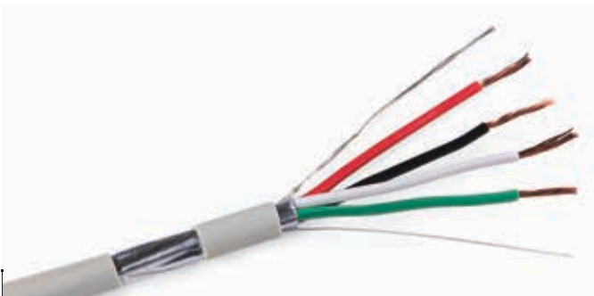
Shielded Multi-Conductor, 16/4, 65 Strand
