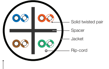
Category 6A 4-Pair, 23 AWG, Solid Plenum Part. No. UTP4-C6A-SOLID-HB2-CMP-XX-305
