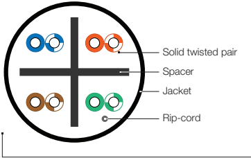
Category 6A 4-Pair, 23 AWG, Solid Riser Available in Shielded Part. No. UTP4-C6A-SOLID-CMR-XX-305
